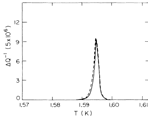
FIG. 26. Predicted widening of the peak due to local finite flow of rotation-induced vorticity.
