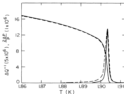
FIG. 16. Solid lines—reduced period and excess dissipation with the cell at rest, for a 30.5-Å film. Dashed lines—reduced period and excess dissipation while rotating at \Omega = 8 rad/sec.
